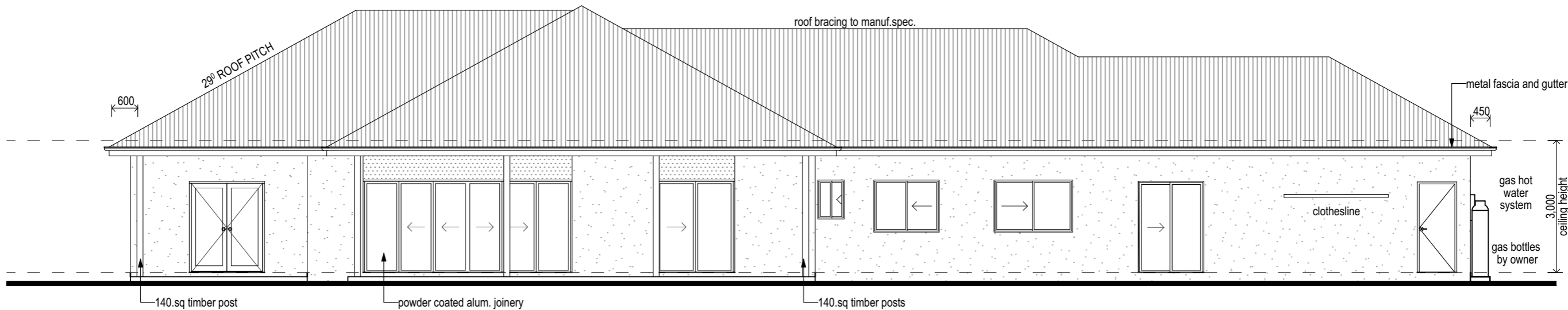
REAR ELEVATION Scale 1:100
