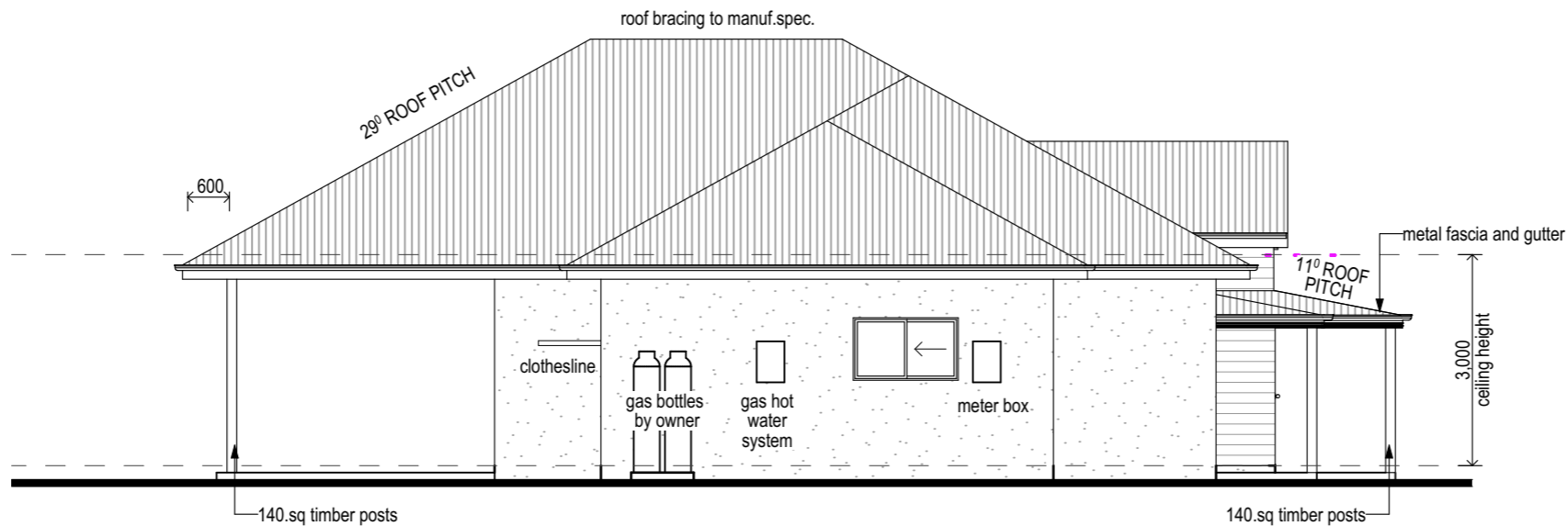
LEFT ELEVATION Scale 1:100
